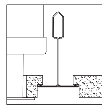
GC2S - 15/16" TEGULAR
