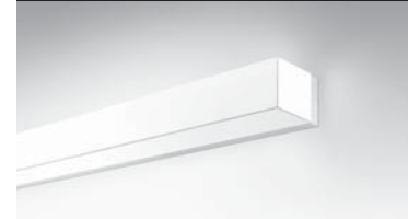
Surface Linear Kubo
