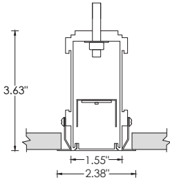
RECOMMENDED CEILING OPENING 2.15"
