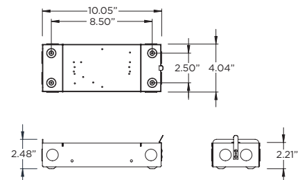
DRIVER ENCLOSURE (PROVIDED BY 3G)
