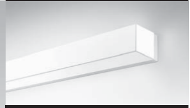
Surface Linear Kubo
